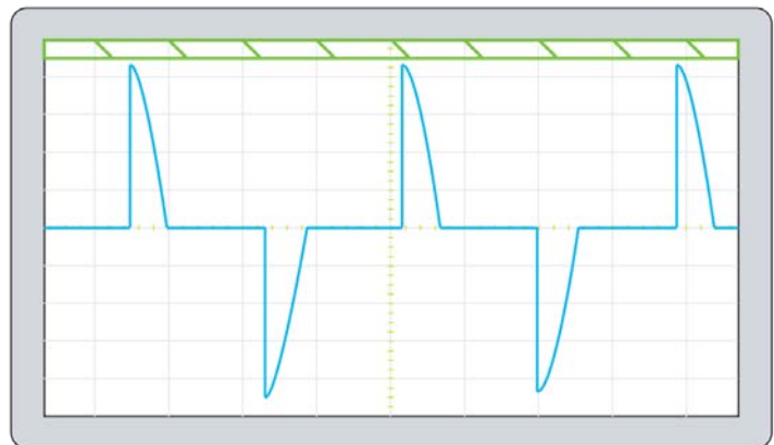
Fig 3. High CF waveform with peak range
