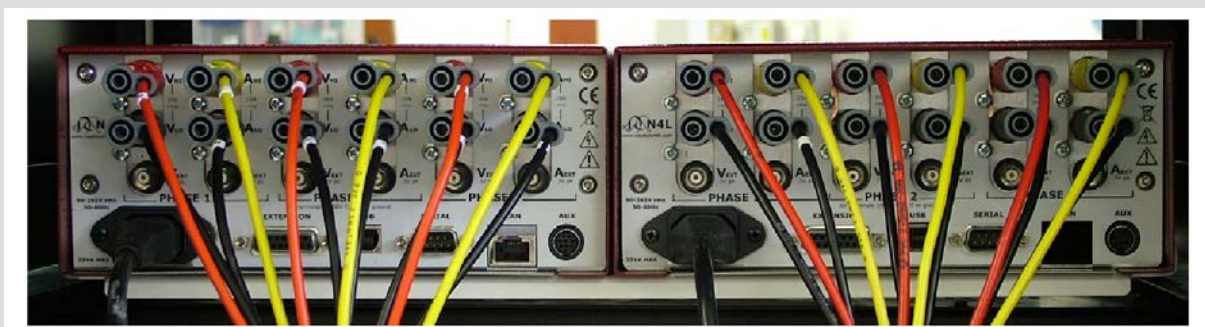
Below depicts the Twin Instrument configuration giving a convenient Six-Phase solution
